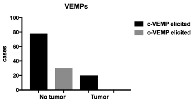
Figure 2. VEMPs according to side. Tumors tended to eliminate VEMP signals: 21% of c-VEMPs and 0% of o-VEMPs were elicited on tumor side. c-VEMP: cervical evoked vestibular myogenic potential; o-VEMP: ocular evoked vestibular myogenic potential.
